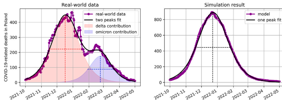
Fig. E.11. Example of fitting the peaks with the logistic distribution, for delta (and omicron ) wave(s) of COVID-19-related deaths in Poland: (a) two-peaks fit to real-world data, (b) one-peak fit to the simulation result. Filled red and blue area in (a) show two contributing peaks. Dashed lines in both panels represent the determined parameters of the peaks: the location of the vertical line for the peak position, its length for the peak value, the length of the horizontal line for the peak width. (For interpretation of the references to color in this figure legend, the reader is referred to the web version of this article.)
