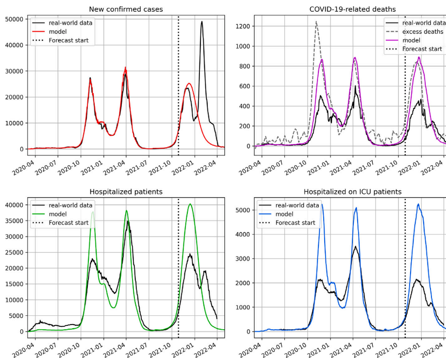
Fig. F.12. Comparison between the PDYN model-generated output (colored lines) and the epidemiological data published by the Polish Ministry of Health (black) and Eurostat (Eurostat, 2023a) (dashed gray) for the entire course of the COVID-19 epidemics in Poland. Top left: new confirmed cases. Top right: COVID-19-related deaths. Bottom left: hospitalized patients. Bottom right: ICU patients. The vertical dotted line indicates the simulation date. (For interpretation of the references to color in this figure legend, the reader is referred to the web version of this article.)
